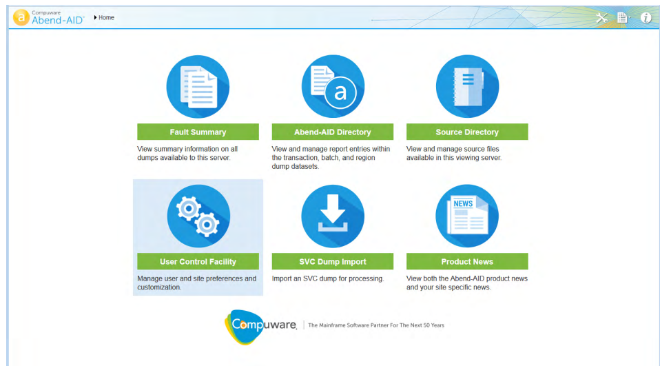
Figure 8. Abend-AID Web Browser Interface Page Layout
